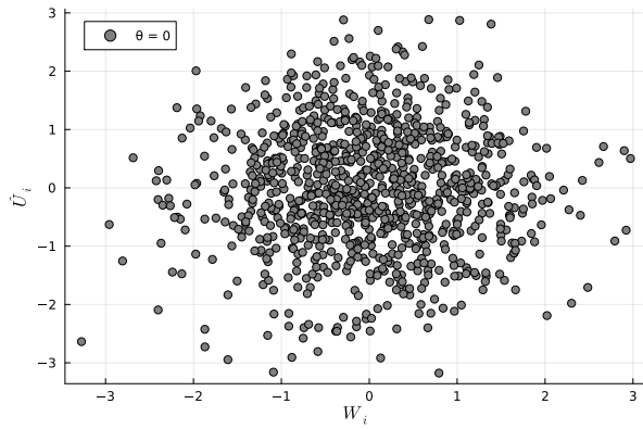
(a) Data under H_0
