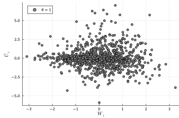
(b) Data under H_1
